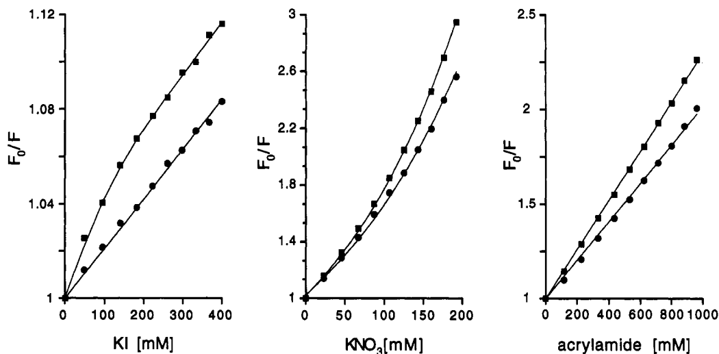
FIGURE 4: Differences in Trp quenchability of Mi-CK dimers and octamers. Fluorescence quenching titrations of 96% octameric (●) and 74% dimeric Mi-CK (■) with KI, \text{KNO}_3 , and acrylamide (Stern–Volmer plots). Dimeric Mi-CK was obtained by TSAC dissociation and subsequent extensive dialysis to remove TSAC substrates. Curves are corrected for ionic strength and inner filter effects (see Materials and Methods).
